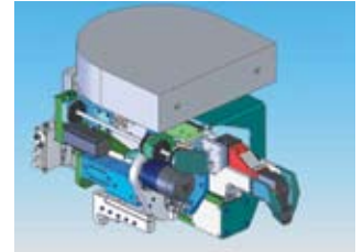
ENDEFFECTOR WITH NUTRUNNER (HILOK)
