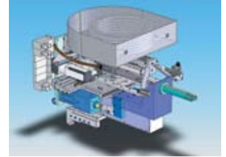
ENDEFFECTOR COLLAR INSTALLATION FOR PULL TYPE (LOCKBOLT)
