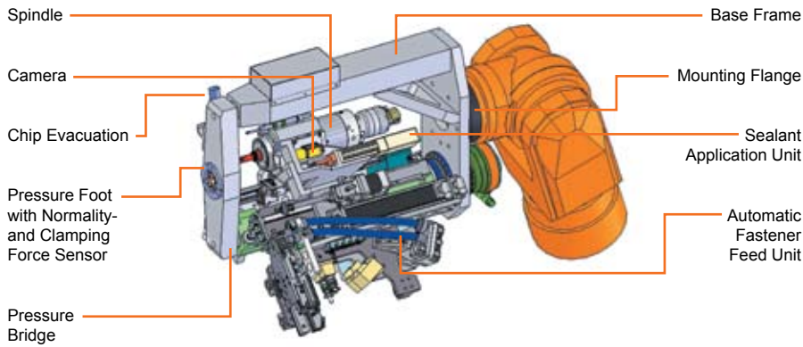
MULTIFUNCTIONAL ENDEFFECTOR
