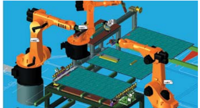
LAYOUT EXAMPLE
